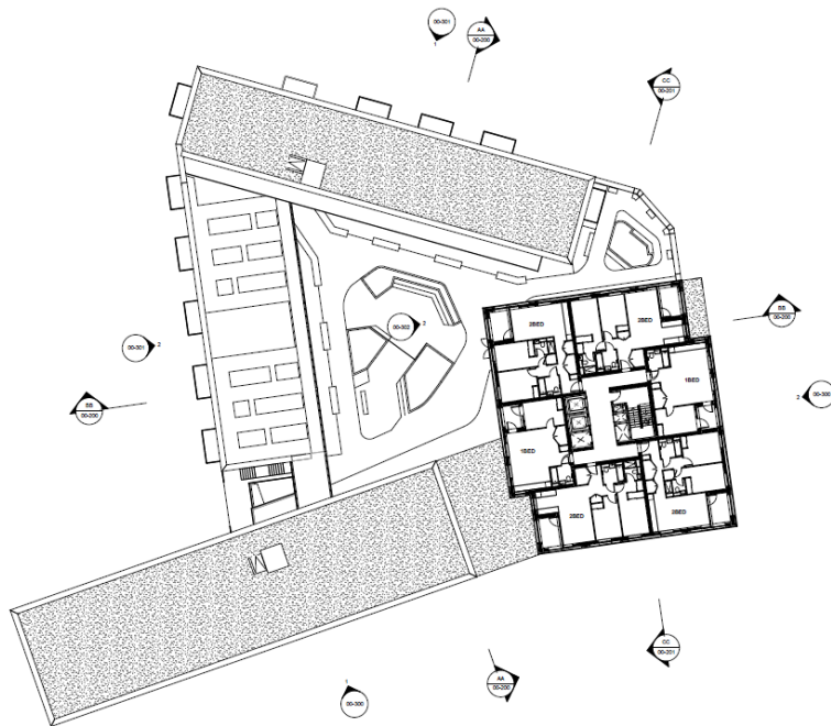
Image 1.10 – Welbourne - Proposed Tenth to Fifteenth Floor Plan
