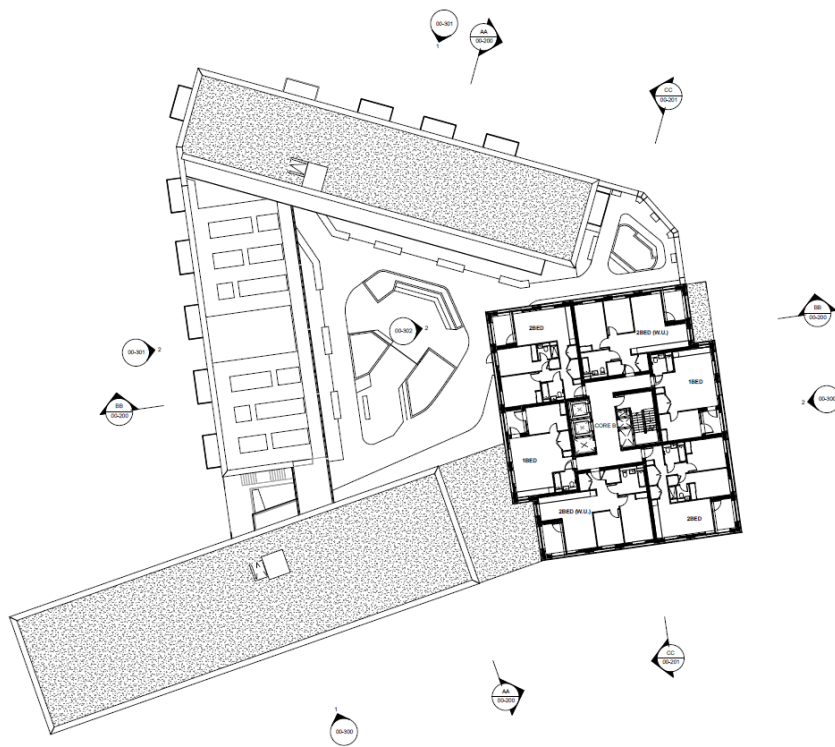
Image 1.7 – Welbourne – Proposed Sixth Floor
