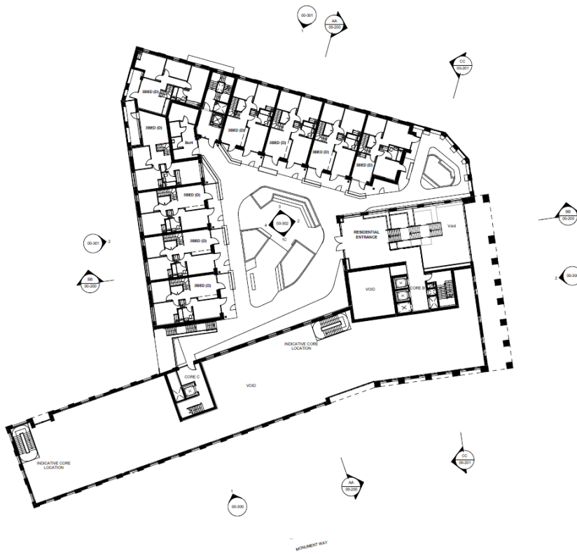
Image 1.2 – Welbourne – Proposed First Floor
