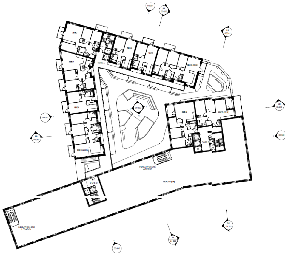
Image 1.3 – Welbourne – Proposed Second Floor
