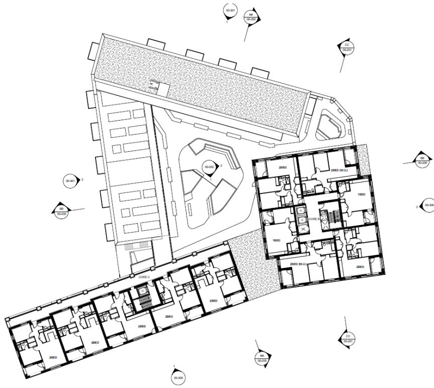
Image 1.7 – Welbourne – Proposed Sixth Floor
