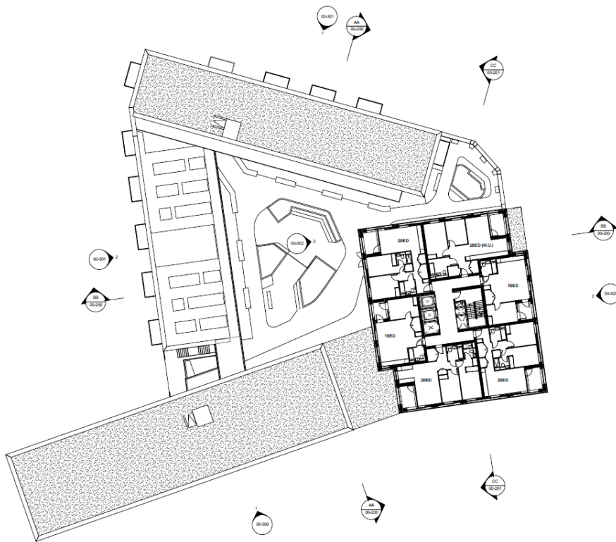
Image 1.9 – Welbourne - Proposed Ninth Floor Plan
